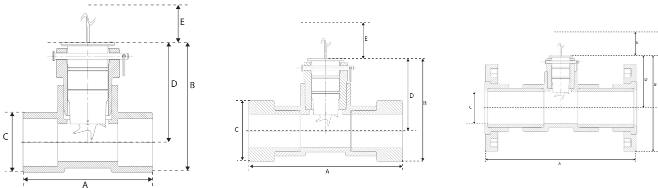
Figure 1: A = Overall Length; B = Overall Height; C = Diameter; D = Center of Tube to Top Height; E = Minimum Clearance for Sensor Removal
