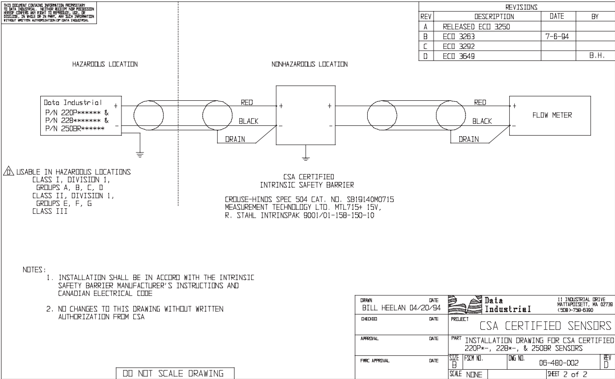
Figure 2: Sample Installation Drawings
