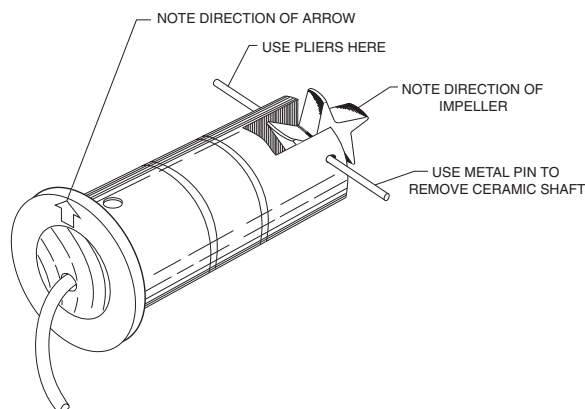
Figure 3: Impeller Assembly and Shaft
